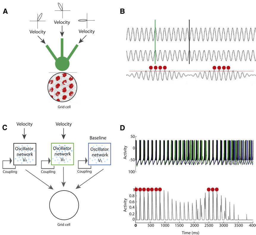
Figure 2. First- and Second-Generation Oscillatory-Interference Models
